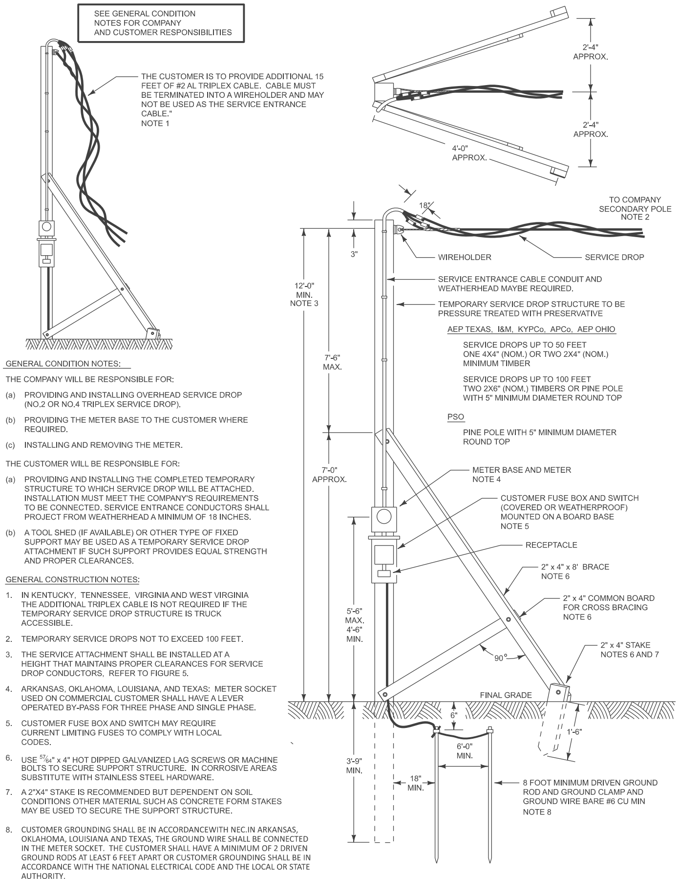
TEMPORARY SERVICE INSTALLATION FROM EXISTING OVERHEAD SECONDARY
