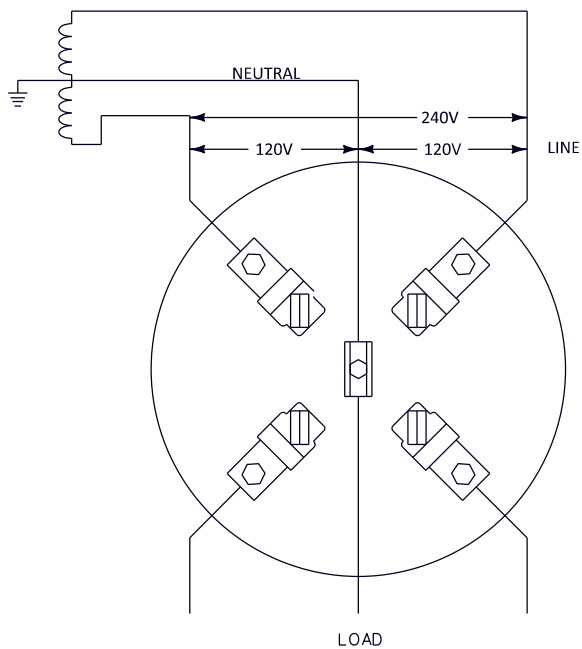
3 WIRE 120/240 VOLT SINGLE PHASE SELF CONTAINED
